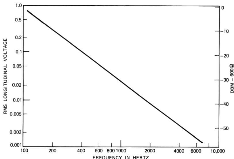
Fig. 1—Longitudinal signal limitations.
